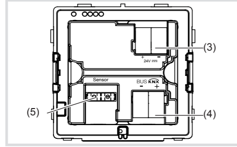
Figure 2: Rear view
